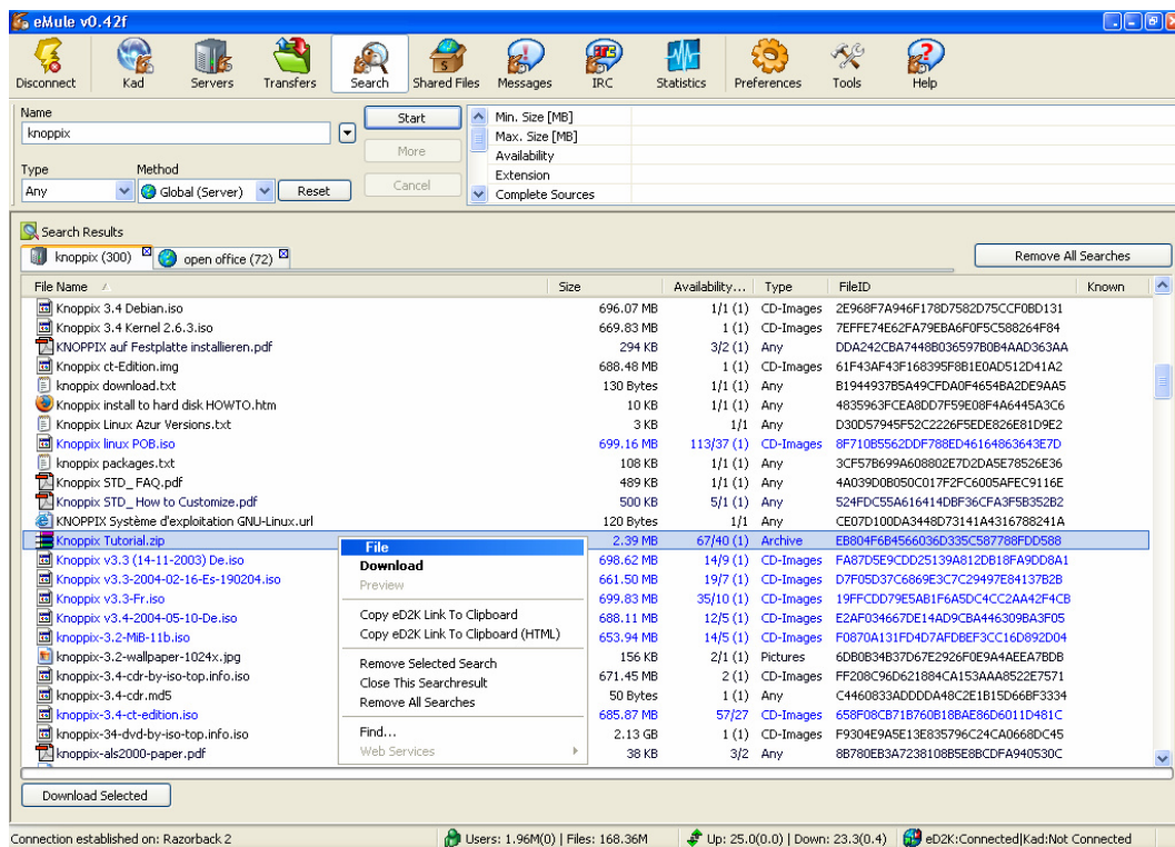
Figura 18: screenshot eMule
