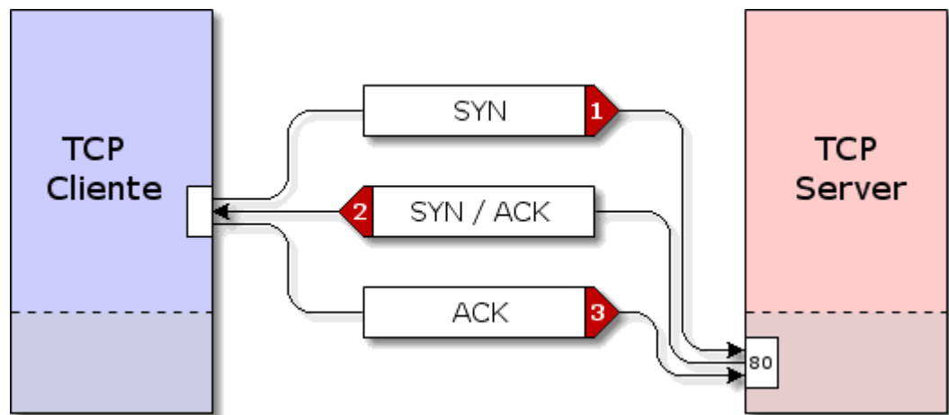
Figura 31: Three-Way Handshake
